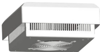
EXTRACTOR . P/ TAB EXT:400X135MM INT:259X259MM 230VAC 870/960M3/H IP54 230VAC Cód. NTLFF230C
